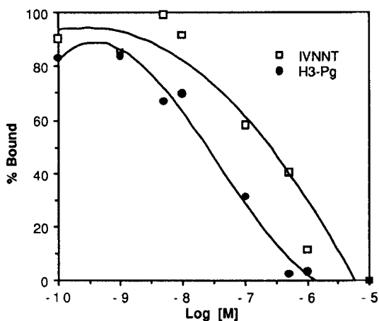
Figure 3. The affinity of the binding of \text{E-}^{125}\text{IVNNT} and [^3\text{H}]\text{R5020} was determined by measuring the binding to T47D cells in the presence of increasing concentrations of unlabeled progesterone ranging from 1 \times 10^{-10} to 1 \times 10^{-5} \text{ M} .
